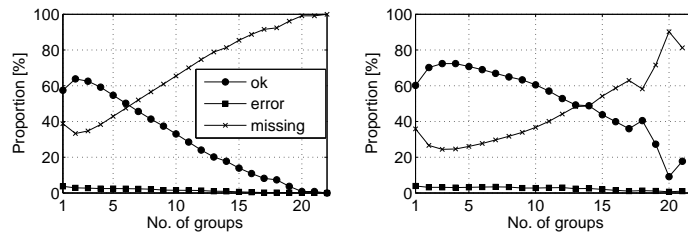
Fig. 2: Prediction results when the data have been divided into 1 . . . 22 group(s). For each grouping, the results are sums of results of all the models corresponding to the grouping. The right panel indicates the the prediction results when the missing predictions of the first variable of each group are ignored. In the left panel, these are taken into account. The legend shown in the left panel is the same for both illustrations.
